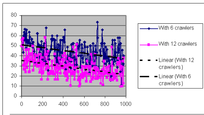
Figure 8.3: Percentage of probes required (compared to the respective brute-force approach) with probing threshold=50msec
