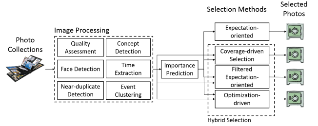
Figure 1: Approach overview of automatic photo selection.
