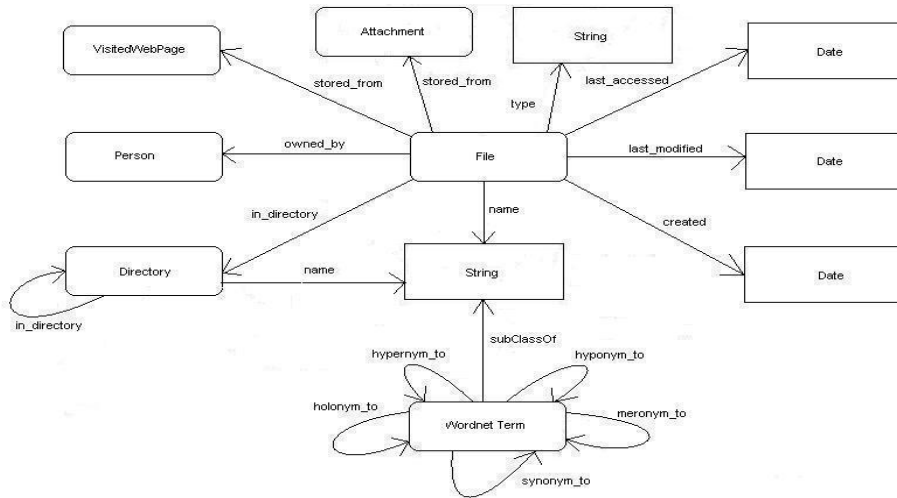
Fig. 2. File prototype
